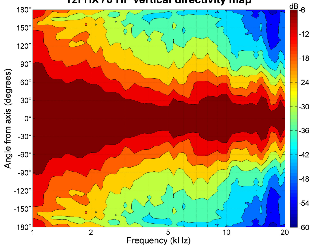
12FHX 76 HF vertical directivity map
