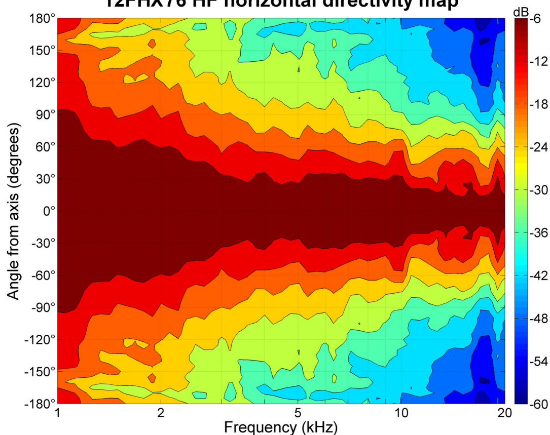
12FHX76 HF horizontal directivity map
