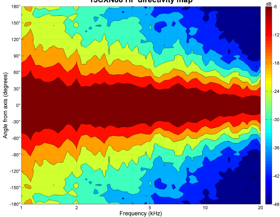
15CXN88 HF directivity map
