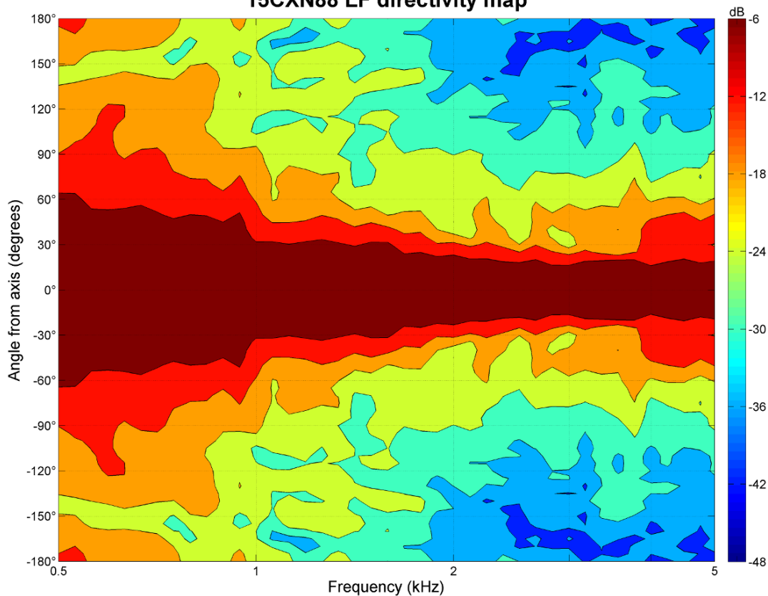
15CXN88 LF directivity map
