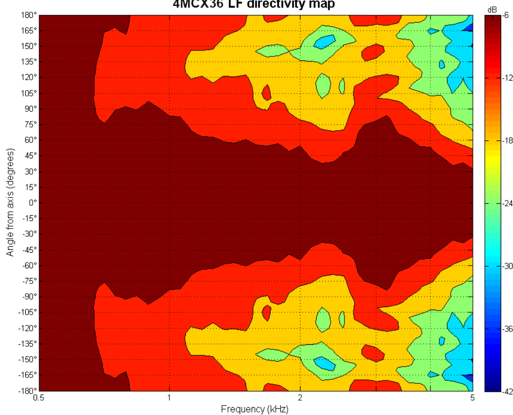
4MCX36 LF directivity map
