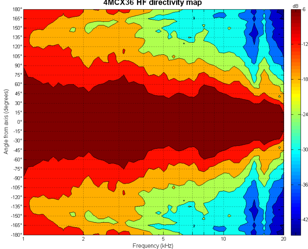
4MCX36 HF directivity map
